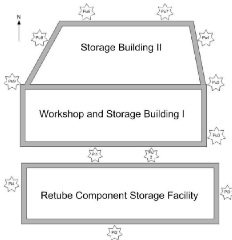
Figure 27. Thermoluminescent Dosimeter Locations around the PWF Phase I site.
